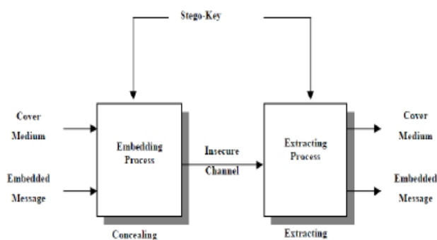
Fig. 1. Steganographic Process
