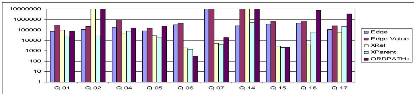
Fig. 2 Read Counts (This diagram shows the number of logical reads or accesses are needed for answering each query in each schema)
