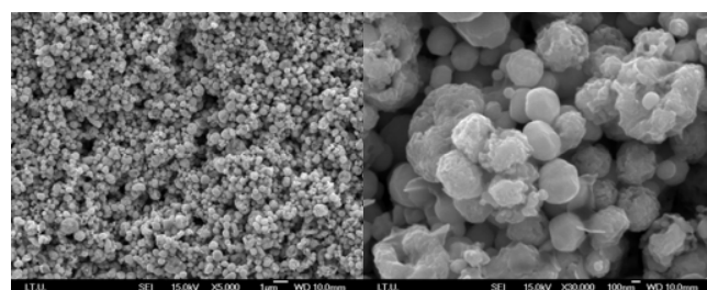
Fig. 4 SEM pictures of Ag/ZnO nanocomposite particles
