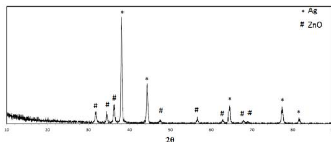
Fig. 3 XRD pattern of Ag/ZnO nanoparticles
