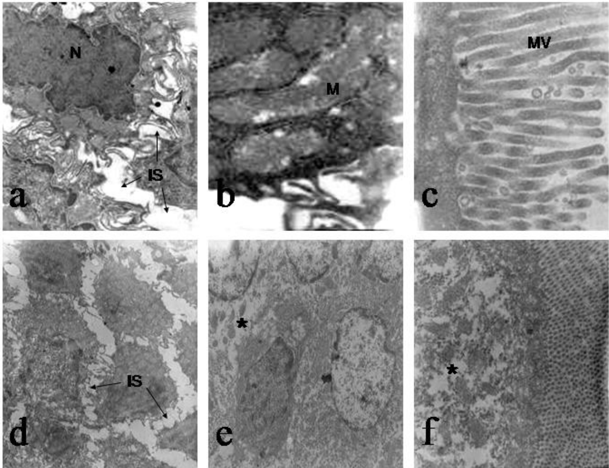
Fig. 3 Transmission electron micrographs of irradiated duodenum mucosa at a dose rate of 1 \text{ Gy}\cdot\text{h}^{-1} , a dose of 2 Gy, 24 h (a, b, c) and 48 h (d, e, f) after irradiation showing dense nucleus with irregular outlines (N), enlarged mitochondria (M), altered brush border microvilli (MV), intercellular spaces (IS) and necrotic areas (asterisk). Magnification: 12,500 X (a, c); 16,200 X (b); 40,000 X (c); 6,400 X (d, e); 16,200 X (f).
