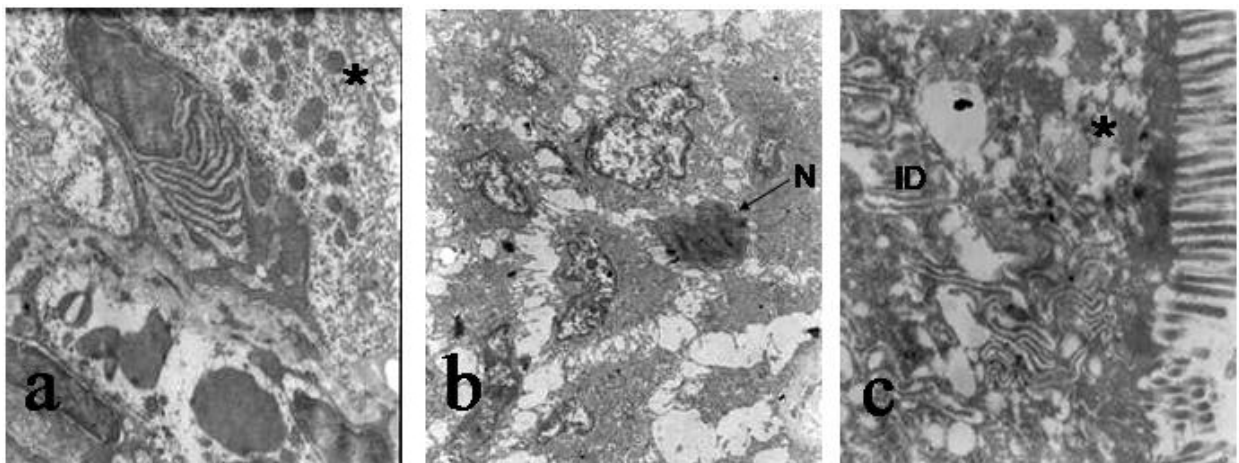
Fig. 4 Transmission electron micrographs of irradiated duodenum mucosa at a dose rate of 1 \text{ Gy}\cdot\text{h}^{-1} , a dose of 4 Gy, 24 h (a, b, c) and 48 h (d, e, f) after irradiation showing large necrotic areas (asterisk) within enterocyte cytoplasm, intercellular spaces and enlarged interdigitations (ID). Magnification: 12,500 X (a, c); 3,950 X (b); 20,000 X (c).
