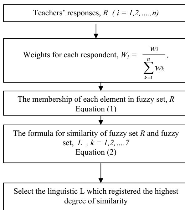
Fig. 1 Measuring procedures based on the fuzzy conjoint model
