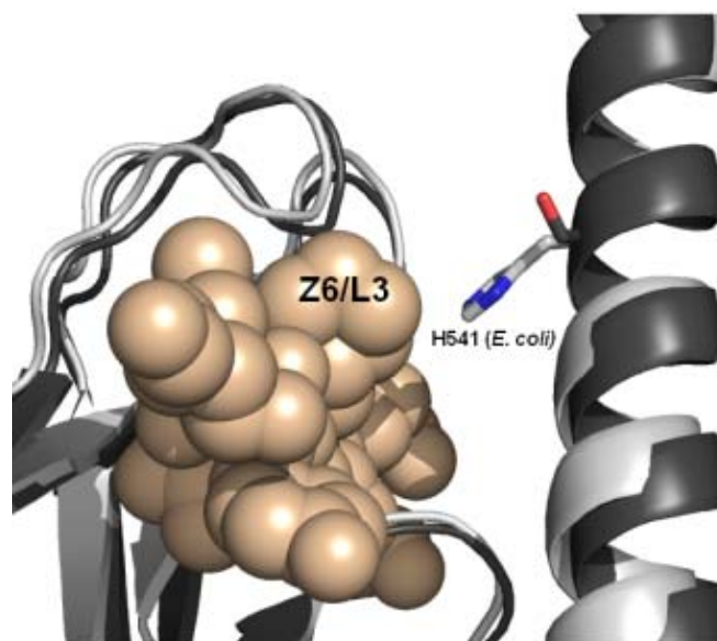
Fig. 4 Superimposition of the crystal structure of the E. coli DnaK complex with a pyrrolicorcin-derived peptide with the homology model of H. pylori DnaK. The inhibitor peptide is drawn in all-atom representation. The side chains of His541 ( E. coli DnaK) and Ser535 ( H. pylori DnaK) are shown.
