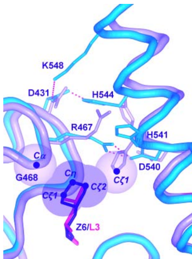
Fig. 3 Superposition of the pyrrolicorcin (carbons in black) and the NR peptide bound to SBD in their respective complexes, showing the broken latch and the additional hydrophobic contacts stabilizing cyclohexylalanine (Z).
