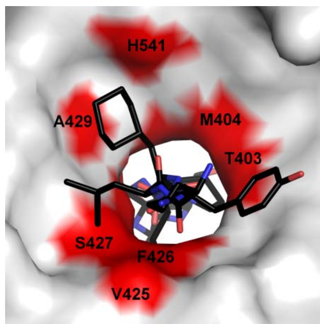
Fig. 2 The pyrrolicorcin binding site of E. coli DnaK. The peptide inhibitor is drawn in a stick representation with carbons in black. The molecular surface of DnaK is shown, and the positions of the residues that form the inhibitor binding site are highlighted in red.
