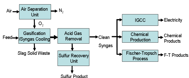
Fig. 1 Block diagram of gasification process and syngas applications
