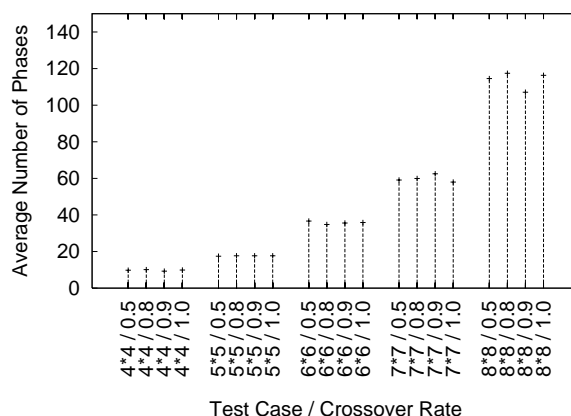
Fig. 8 The average number of phases needed to find a solution for successful runs with crossover rate varying from 0.5 to 1.0
