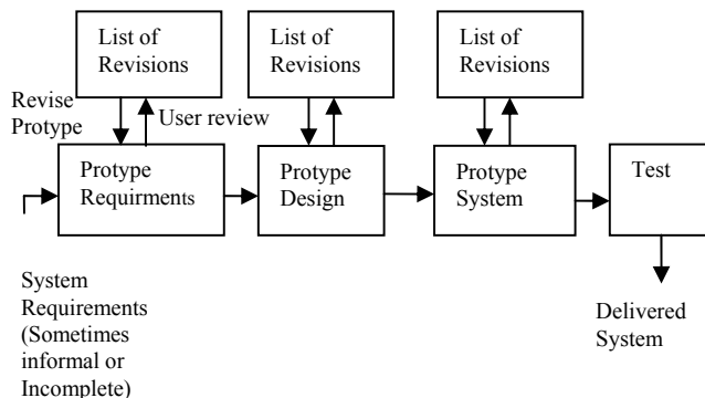
Fig. 4 Iterative Method Outline
