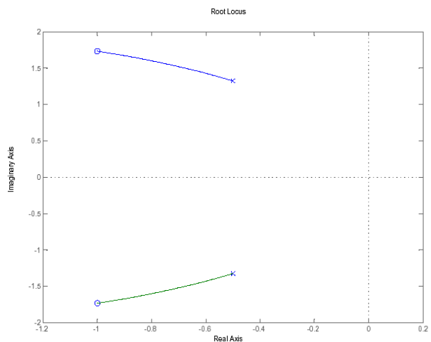
Fig. 8 Root locus of the closed loop system
