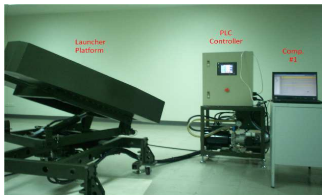
Fig. 1 The Platform of MLRS
