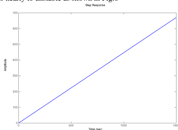
Fig. 5 Step response of the open loop system
