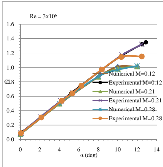
Fig. 4 Drag coefficient vs AoA for clean GLC305 airfoil
