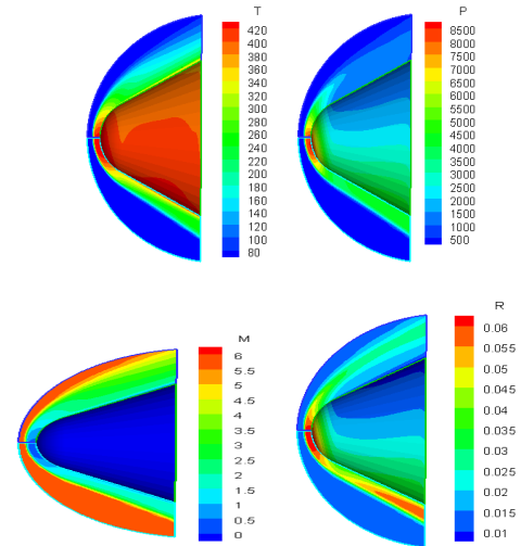
Fig. 10 Contours of temperature, pressure, mach no., and density at Mach 5.9, r_n/r_b = 0.5 and angle of attack 12°
