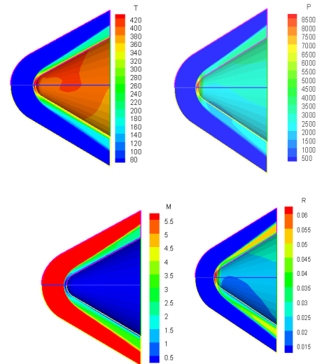
Fig. 11 Contours of Temperature, pressure, Mach no. and density at \theta=30^\circ , r_n/r_b=0.25 and angle of attack -4^\circ
