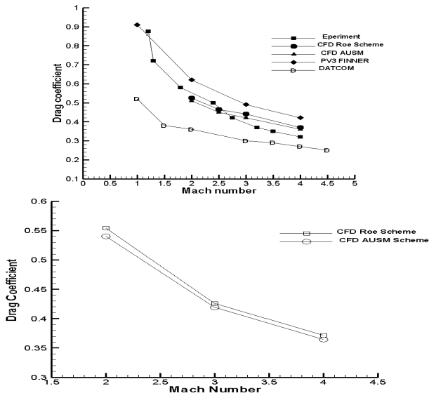
Fig. 8 Drag coefficient of finned missile at zero and 1° angle of attack.
