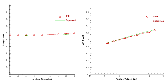
Fig. 14 Graph for Drag coeff. , lift and Pitching moment Coefficient for r_n/r_b=0.25 and \theta=30^\circ
