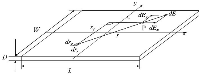
Fig. 1 Model of a rectangular charged area
