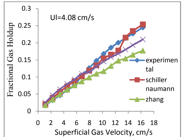
Fig. 2 Comparison of fractional gas holdup calculated by different drag models with experimental value
