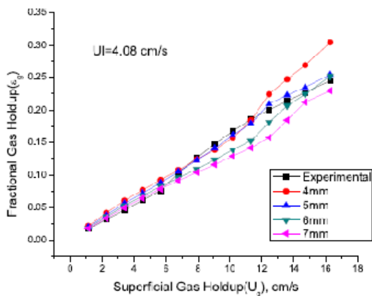
Fig. 1 Effect of bubble diameter over gas holdup
