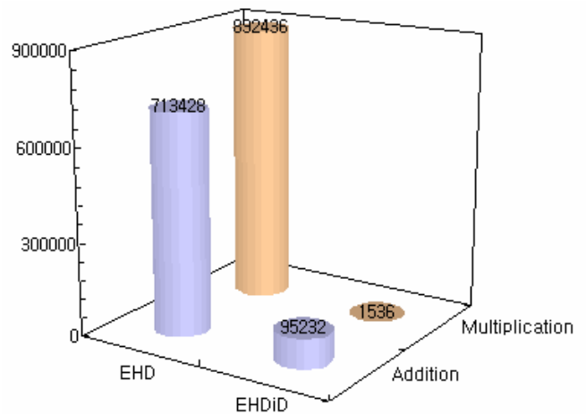
Fig. 7 Comparison of complexity between EHD and EHDiD
