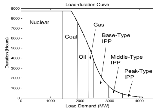
Fig. 1 Load Duration Curve
