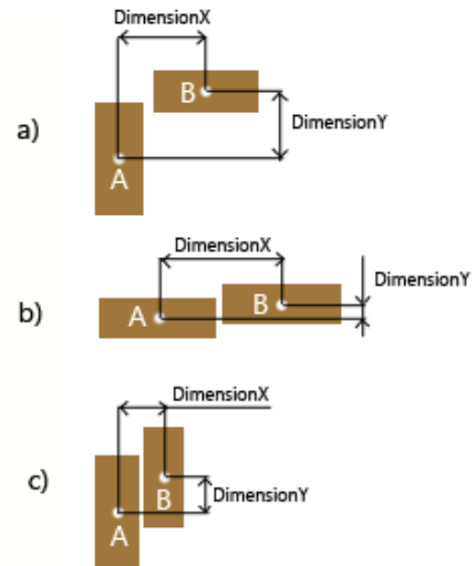
Fig. 8 Collision control between: a) 90° and 0° orientation of the prisms b) 0° and 0° orientation of the prisms c) 90° and 90° orientation of the prisms
