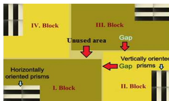
Fig. 3 Steudls algorithm [7]
