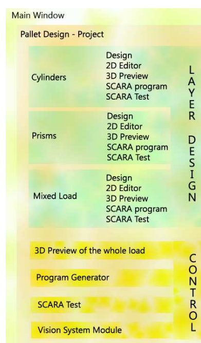
Fig. 1 Software structure
