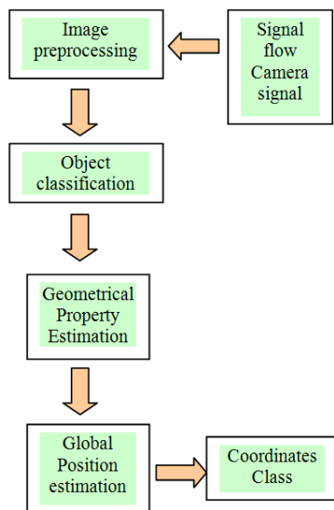
Fig. 16 Vision algorithm
