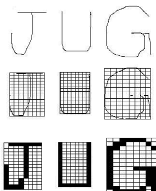
Fig. 3 Steps in Feature Extraction
