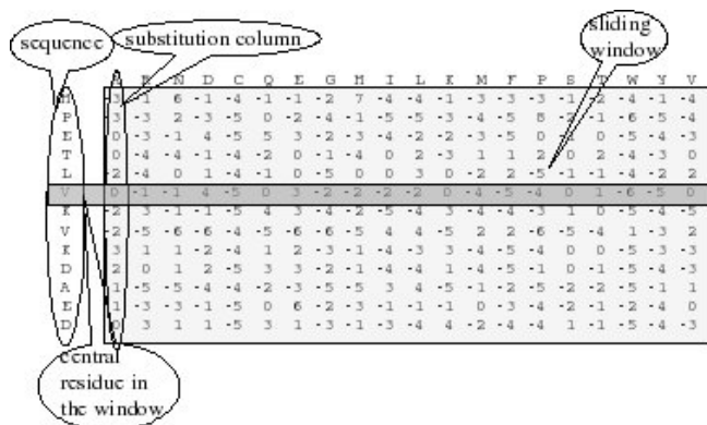
Fig. 1: Sliding window on the PSSM matrix.
