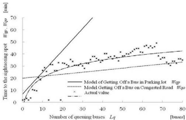
Fig. 8 Relationship between time to the sightseeing spot and number of queuing buses
