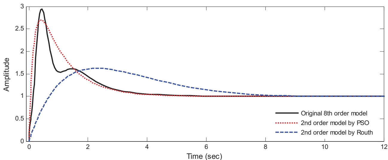
Fig. 5. Step Responses of original system and reduced model of example-2
