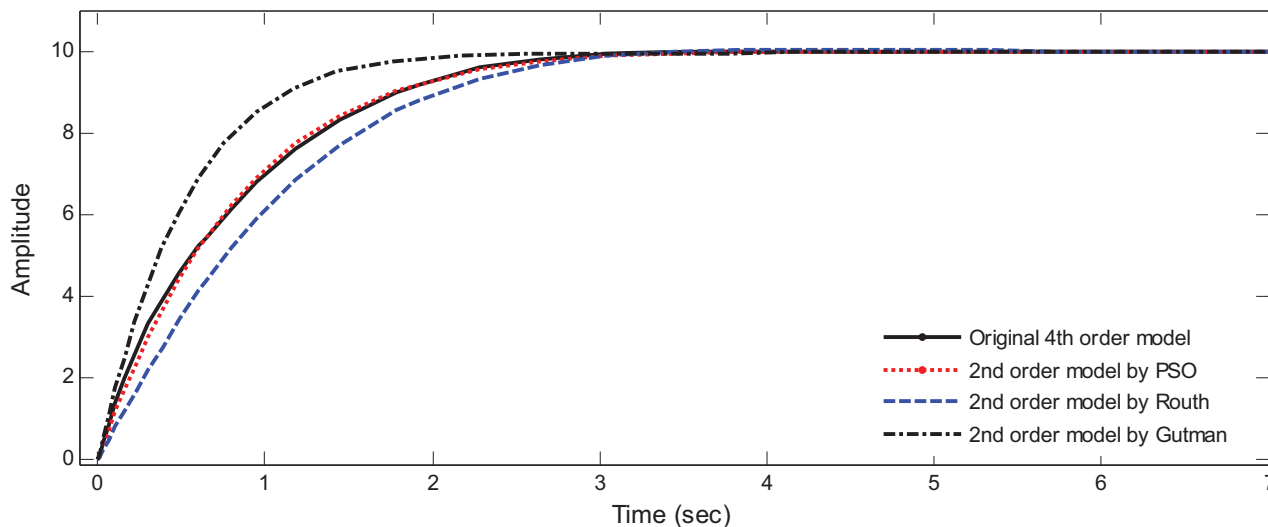
Fig. 4. Step Responses of original system and reduced model of example-1
