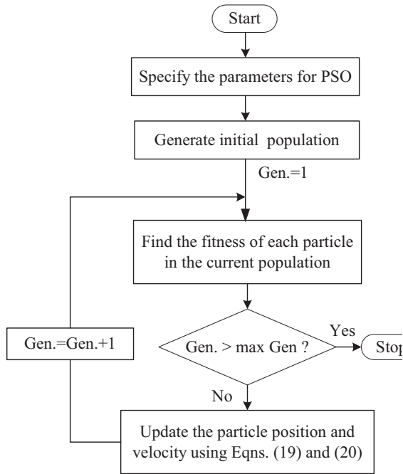
Fig. 2. Flowchart of PSO for order reduction
