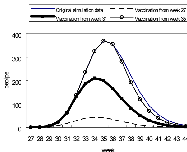
Fig. 9 Vaccination policy starting from different time
