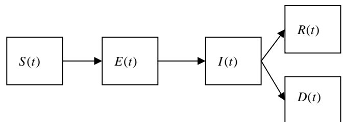
Fig. 2 SEIRD Model
