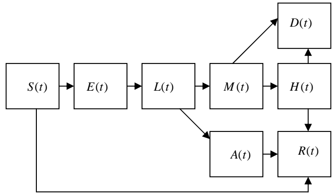
Fig. 4 SELMAHRD model
