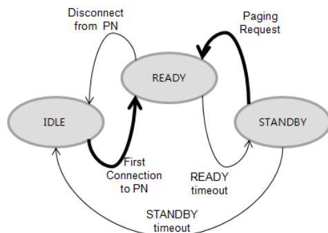
Fig. 3 UE State on 3G mobile network
