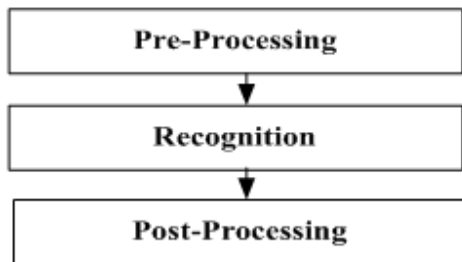
Fig. 1 OCR process [1]
