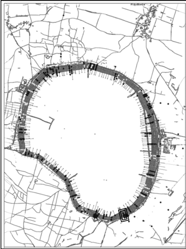
Fig. 3 Plan view of the Želazny Most tailing dam – the black dots show the locations of the CPTs performed and the light grey dots show the locations of the CPTs used in further analysis
