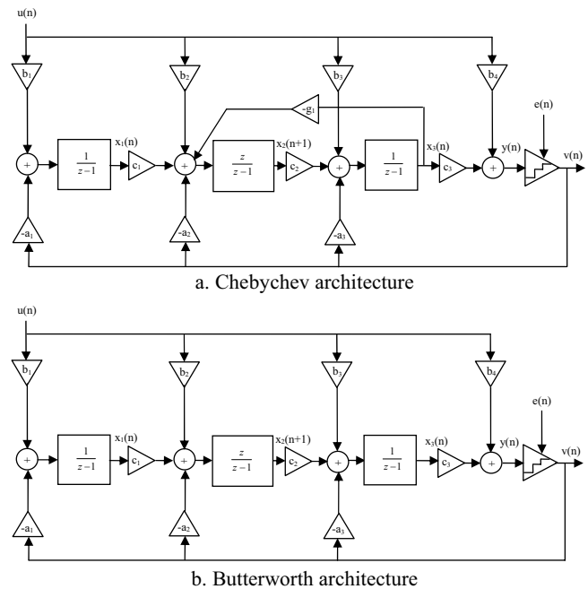
Fig. 7 3 rd -order multibit delta sigma modulators
