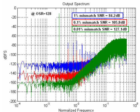
Fig. 17 PSD of the single loop (5-bit) at OSR of 128 for different current mismatches
