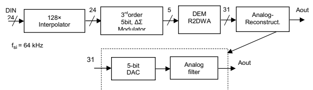
Fig. 1 Multibit delta-sigma DAC signal flow diagram
