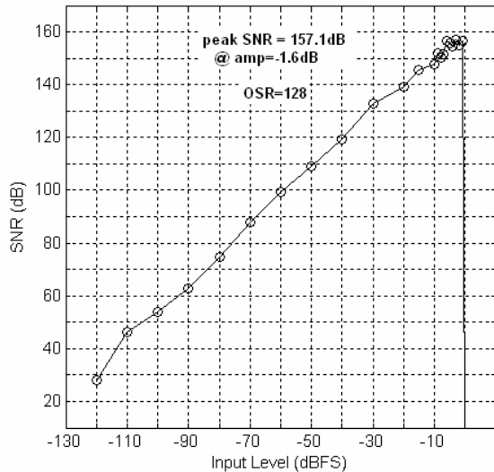
Fig. 14 Ideal SNR vs. input amplitude curve
