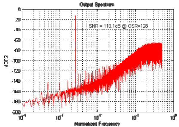
Fig. 16 Illustration of tones behavior of DWA
