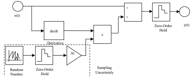
Fig. 19 Modeling a random sampling jitter
