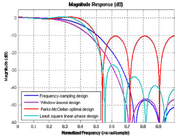
Fig. 2 FIR filter design methods frequency responses
