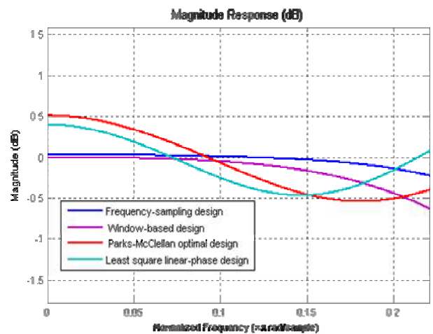
Fig. 3 Zoomed passband
