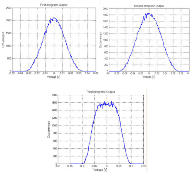
Fig. 9 Integrator output swings
