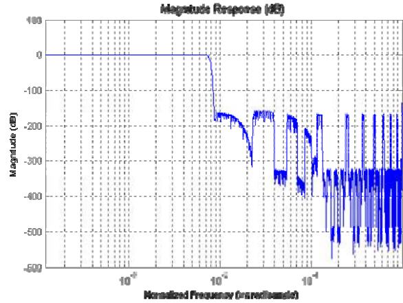
Fig. 6 Magnitude response of the interpolation chain, OSR = 128
