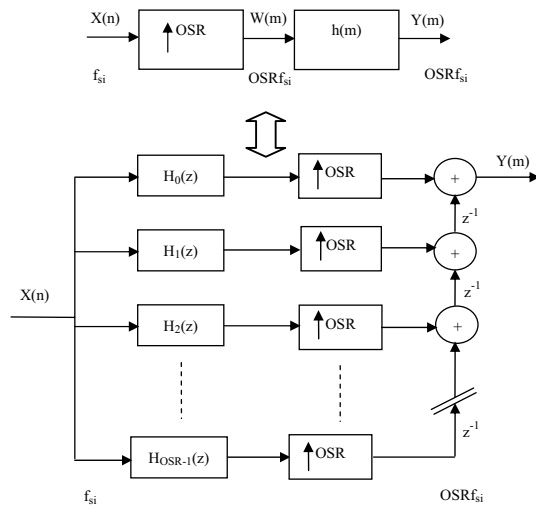
Fig. 4 Polyphase interpolation
