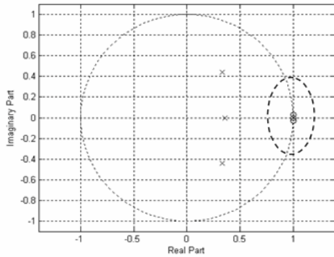
Fig. 8 Pole/zero plot
