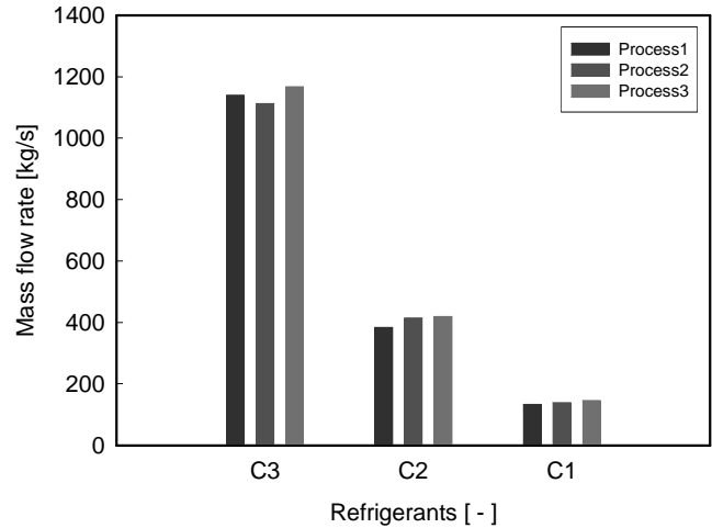
Fig. 4 Comparison of refrigerant mass flow rate
