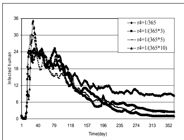
Fig. 11 Model outputs display the time distribution of infected human for the different rate at which the recovered human relapses back to the susceptible human in each district. There are 3 villages in each district; 20 houses in each village. The other parameters are same as Fig. 3 except r_4
