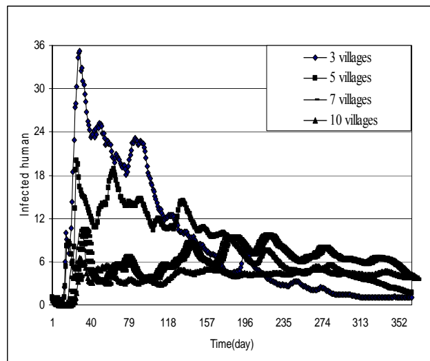
Fig. 3 Model outputs display the time distribution of infected human for the different number of villages in each district. The parameters in our model are r_1 = 1/14 , r_2 = 1/(365*3) , r_3 = 1/(25) , r_4 = 1/(365*10) , r_5 = 1/3 , \gamma = 0.55 , \beta = 0.45 , \mu_v = 0.04 , M = 1,000 , c = 365
