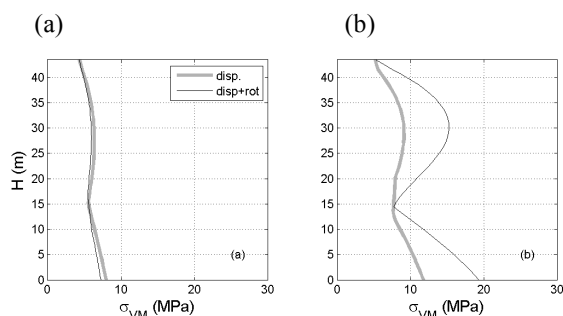
Fig. 4 Comparison of the distribution of maximum Von Mises stress along the tower's height with or without rotational input for records: (a) no.12 and (b) no.18
