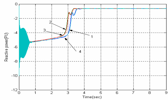
(c) Reactive power
