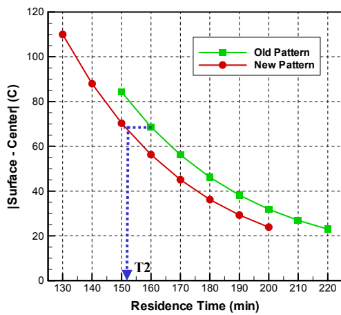
(b) Temperature uniformity inside the slab
