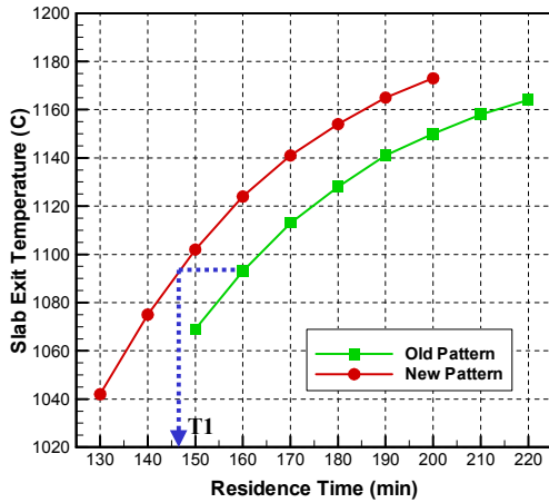
(a) Slab temperature at the furnace exit
