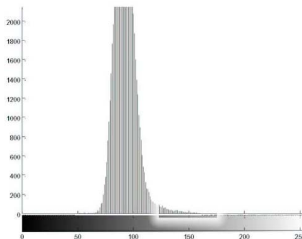
Fig. 5 Histogram of Faulty (Scratch) Fabric
