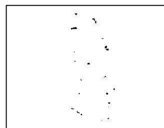
Fig. 11 Binary Image
