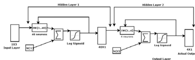
Fig. 9 Design of Feed Forward Back propagation Neural Network
