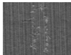
Fig. 10 Grayscale Image
