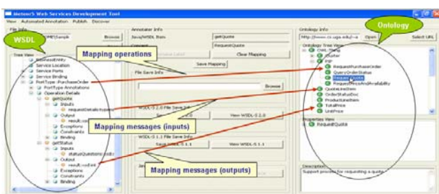
Fig. 3 Annotating Web services with ontological concepts
