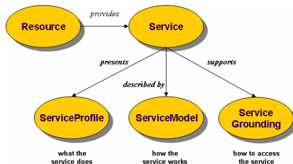
Fig. 4 Organization of OWL-S into modules
