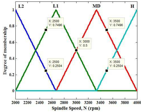
Fig. 2 Fuzzification of spindle speed
