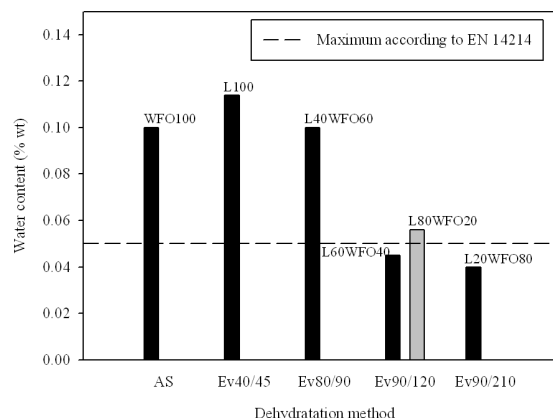
Fig. 1 Water content of biodiesel using different dehydration treatments (nomenclature in the bars refers to sample used and considers percentage of waste frying oil (WFO) and lard (L) used as the raw material)
