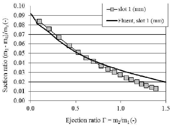
Fig. 8 Suction ratio for various ejection ratio
