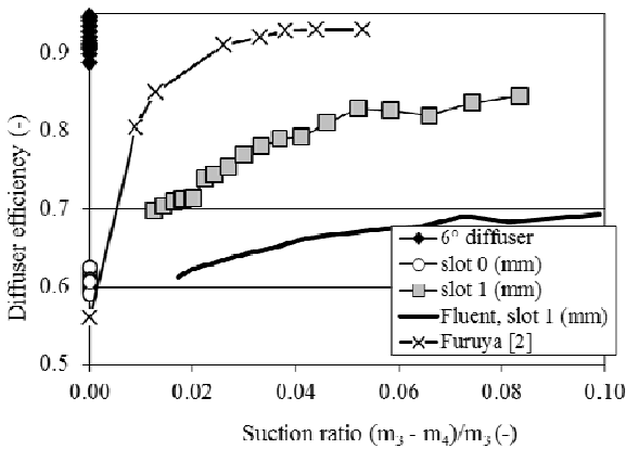
Fig. 9 Diffuser efficiency as a function of suction ratio
