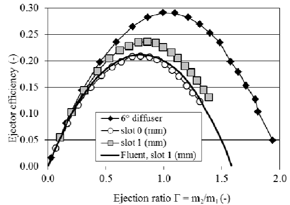
Fig. 3 Ejector efficiency obtained experimentally and numerically for different configuration of the diffuser of the ejector
