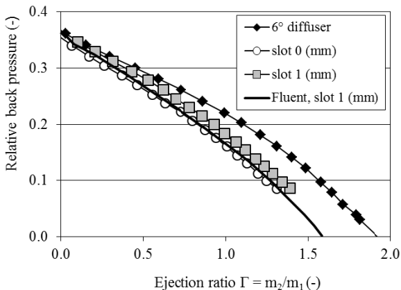
Fig. 6 Relative back pressure (p_4 - p_{02}) / (p_{01} - p_{02}) behind the diffuser for different configuration of the diffuser of the ejector
