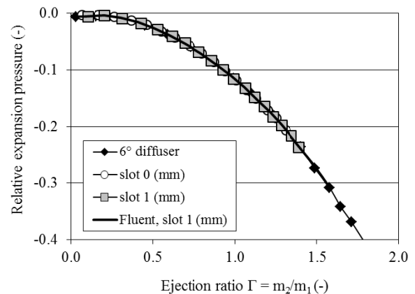
Fig. 4 Relative expansion pressure (p_{12} - p_{02}) / (p_{01} - p_{02}) in the beginning of the mixing chamber for different configuration of the diffuser of the ejector
