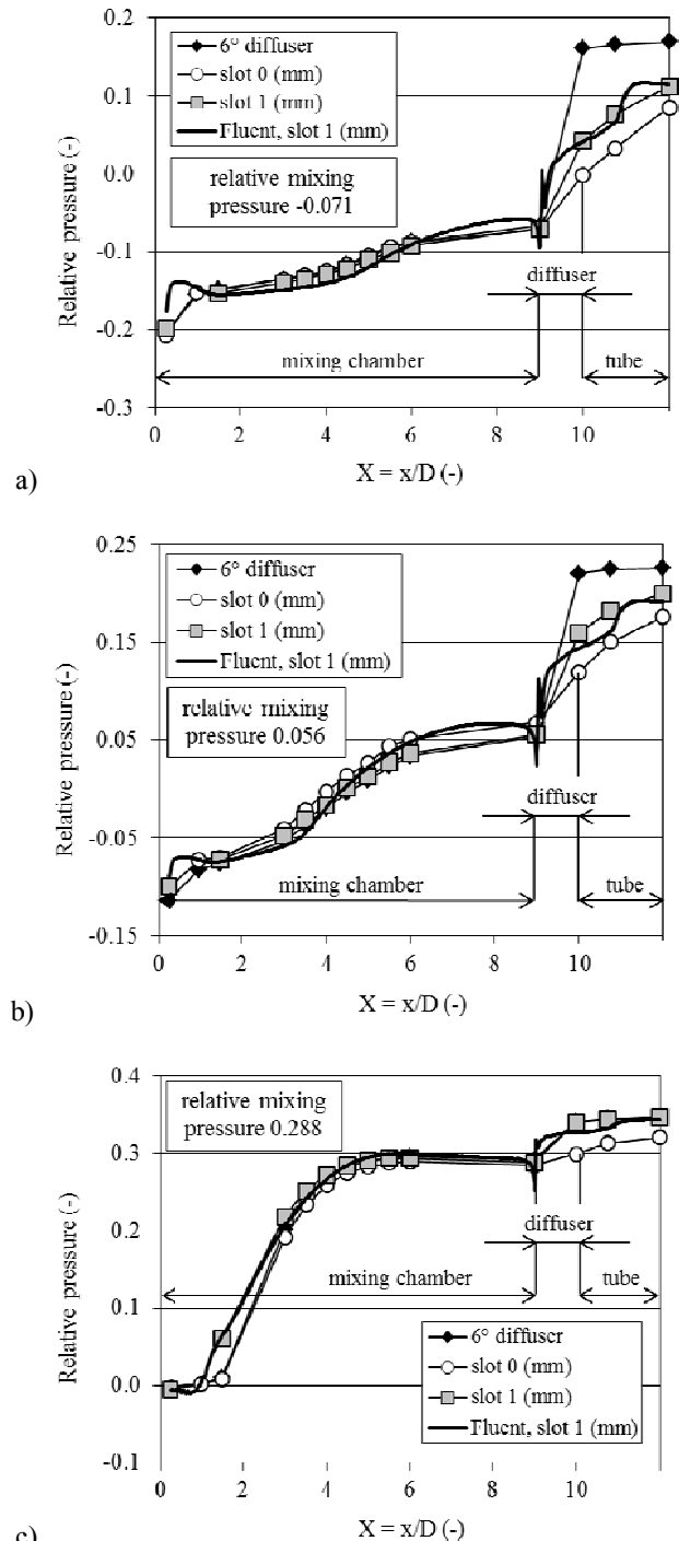
Fig. 10 Static pressure distribution on the mixing chamber wall, diffuser and tube behind the diffuser for three values of mixing pressure. Relative pressure is defined as (p - p_{02}) / (p_{01} - p_{02}) . X = x/D is dimensionless axial coordinate
