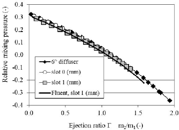
Fig. 5 Relative mixing pressure (p_3 - p_{02}) / (p_{01} - p_{02}) at the end of the mixing chamber for different configuration of the diffuser of the ejector
