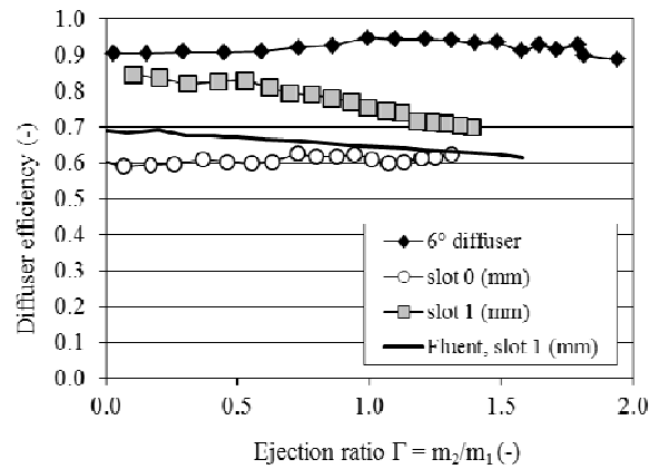
Fig. 7 Diffuser efficiency for back pressure measured 300 (mm) behind the diffuser
