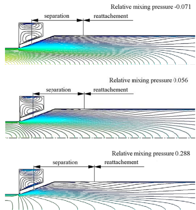
Fig. 12 Contours of axial velocity in the diffuser part of the ejector
