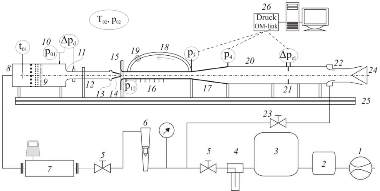
Fig. 2 Experimental arrangement: 1 - compressor, 2 - air dryer, 3 - tank, 4 - filter, 5 - reduction valve, 6 - rotameter, 7 - Coriolis mass flow meter, 8 - stilling chamber, 9 - stilling riddles, 10 - measuring of primary stagnation pressure p_{01} , 11 - measuring of primary mass flow rate, 12 - primary flow supply tube, 13 - holder of primary nozzle, 14 - primary nozzle, 15 - secondary nozzle, 16 - mixing chamber with static pressure taps, 17 - diffuser with suction slot, 18 - suction tube, 19 - velocity probe, 20 - outflow pipe, 21 - measuring of total mass flow rate, 22 - suction ejector, 23 - control valve, 24 - choking, 25 - base, 26 - pneumatic measuring.
