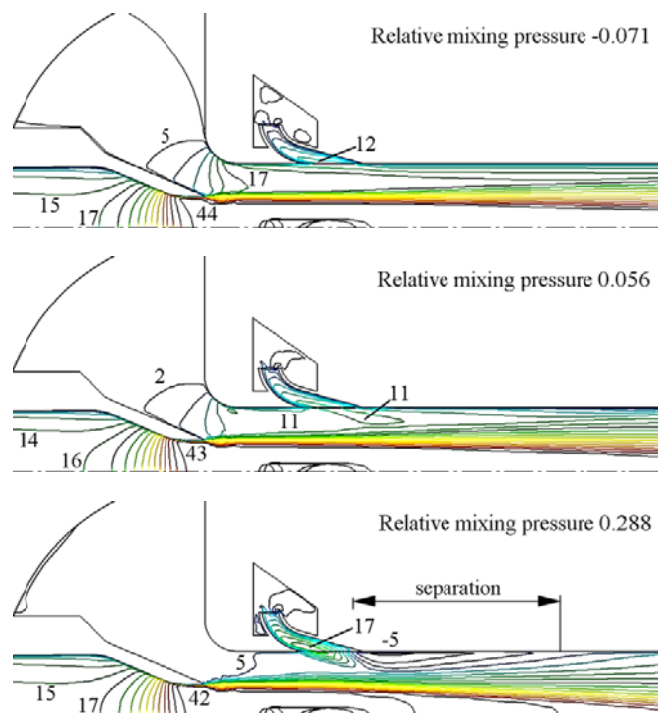
Fig. 11 Contours of axial velocity in the inlet part of the ejector
