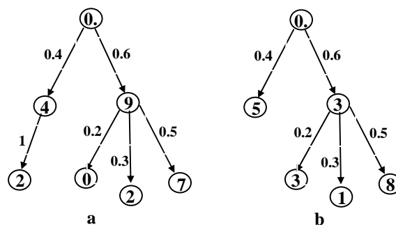
Fig. 2 a. a Digital 2-Complete Probability Tree. b. a Digital Probabilistically Complete Tree
