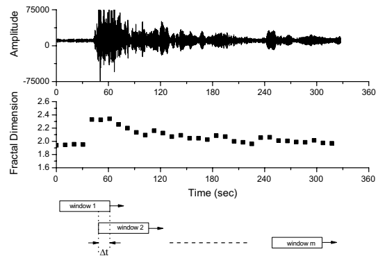
Fig. 4. Typical of successive event of explosion earthquakes and harmonic tremor and its temporal change of fractal dimension. The fractal dimension was estimated based on CEM with TDFD.
