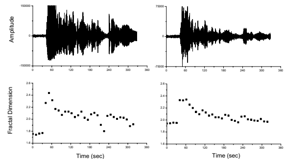
Fig. 6. Similar with Fig. 5 for event occurred on 2005:03:15 00:05.
