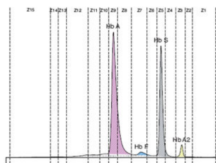
Fig. 2 Electrophoretic profile with varying heterozygous (HbS)
