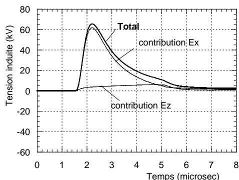
Fig. 9 Induced over voltages calculated by Taylor model
