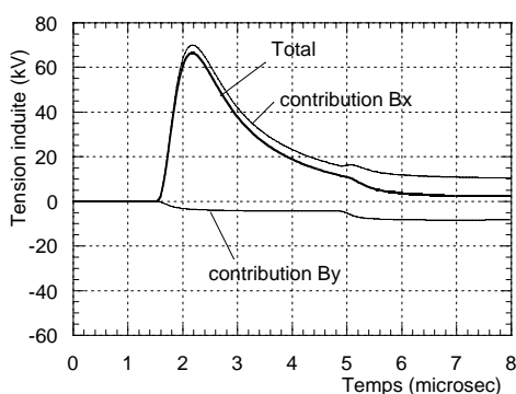
Fig. 10 Induced over voltages calculated by Rachidi Model
