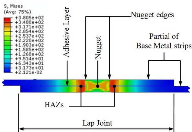
Fig. 9 Contour residual stresses for FE weld-bonded model
