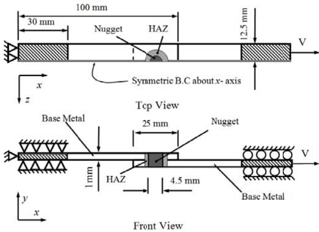
Fig. 4 Spot Weld Model
