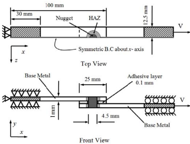
Fig. 5 Weld-Bonded Models
