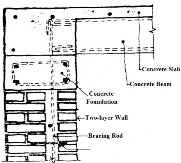
Fig 15 Attaching a two-layer wall to ceiling
