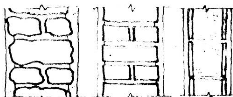
Fig 13 Two-layer wall constructed by new construction material
