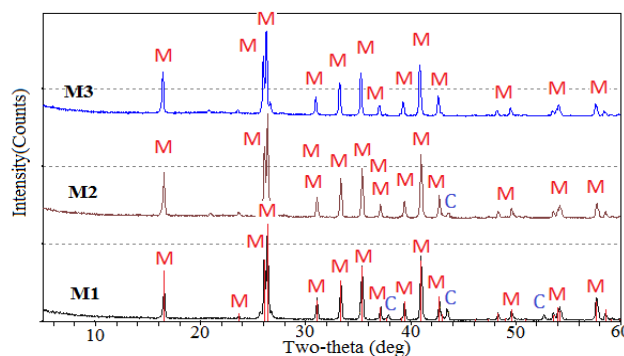
Fig. 6 XRD patterns: Comparison of phases of M series samples. (M- Mullite, C-Corundum)
