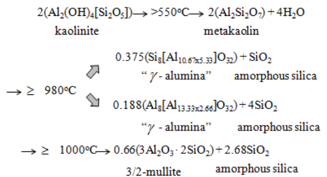
Fig. 1 Kaolinite phases transformation in the time of kaolin heating [6]
