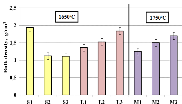
Fig. 8 The bulk density of samples after sintering
