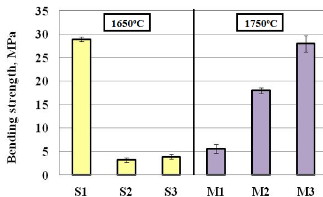
Fig. 10 The bending strength of samples
