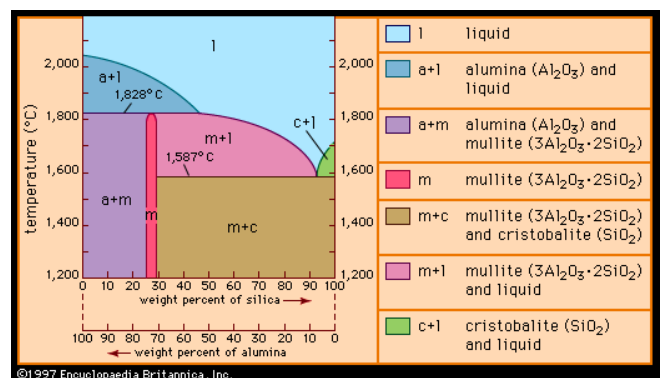
Fig. 2 Phase diagram of the alumina-silica system. Dependence on the temperature, on the content of silica and alumina quantity [7]
