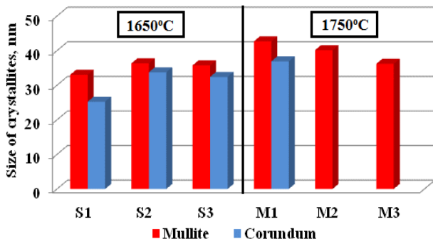
Fig. 11 Sizes of mullite and corundum crystallites, (nanometer)
