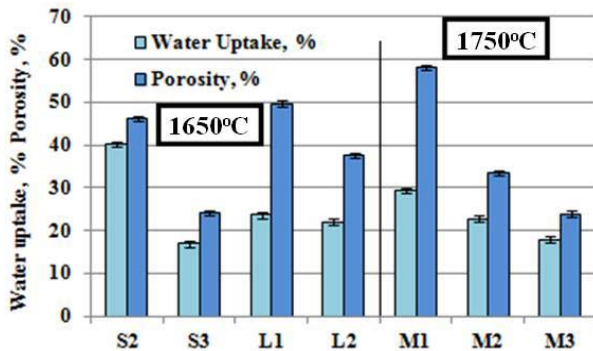
Fig. 12 Water uptake and porosity of samples
