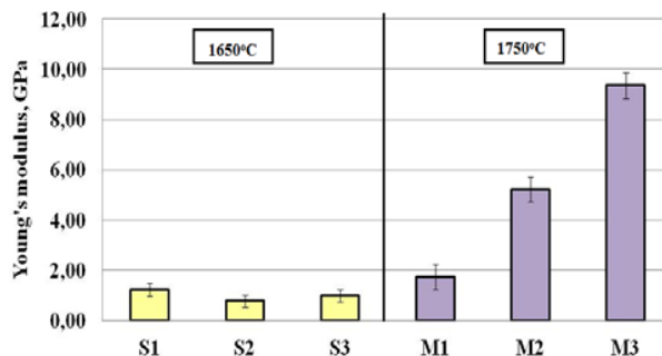
Fig. 9 The Young's modulus of samples
