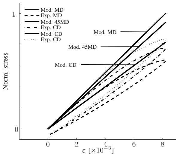
Fig. 6. Prediction and experimental response in in-plane tension. The given experimental data are each averaged from nine specimens, respectively. The scatter is \pm 5MPa .
