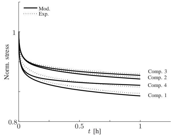
Fig. 3. Prediction and experimental response in out-of-plane relaxation for repeated compression and relaxation behaviour of one stack of samples. The stack is put at rest (meaning not subjected to any load) for 5 min in between each compression/relaxation w.r.t. Comp. 1-3. The rest between compression/relaxation Comp. 3 and 4 is 264h.
