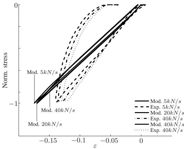
Fig. 5. Prediction and experimental response in out-of-plane compression.
