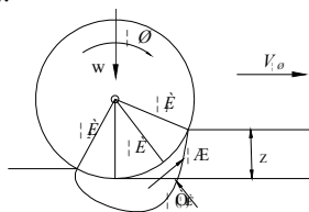
Fig. 5 Rigid Wheel—Lunar Surface Interaction Model
