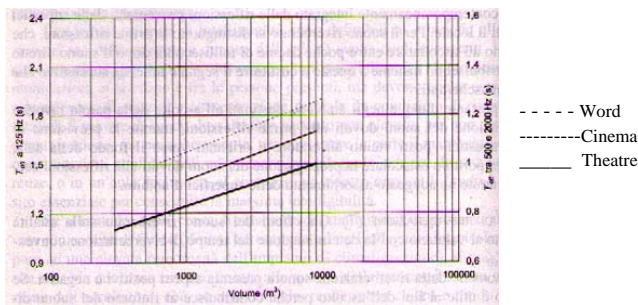
Fig. 46 – Optimal values of reverberation time
