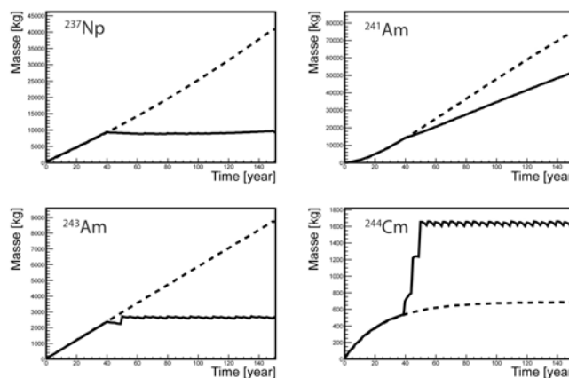
Fig. 8. Masse evolution of the major Minor Actinide between the two case scenario, where dashed line correspond to the pure PWR scenario and plain line to the PWR+ADS scenario, on the top left one find ^{237}\text{Np} , with the top right ^{241}\text{Am} , on the bottom left ^{243}\text{Am} and on the bottom right ^{244}\text{Cm} .
