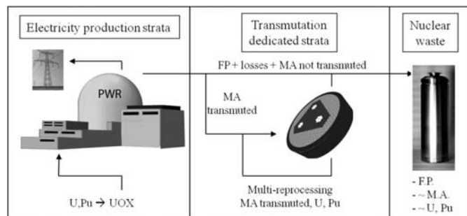
Fig. 3. Schematic double strata scenario, with from left to right, the electricity production, the Minor Actinide transmutation, ultimate nuclear waste.
