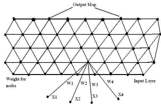
Fig. 6. Self Organizing Feature Map
