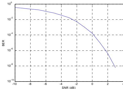
Fig. 5 BER of standard zigbee system (IEEE 802.15.4)
