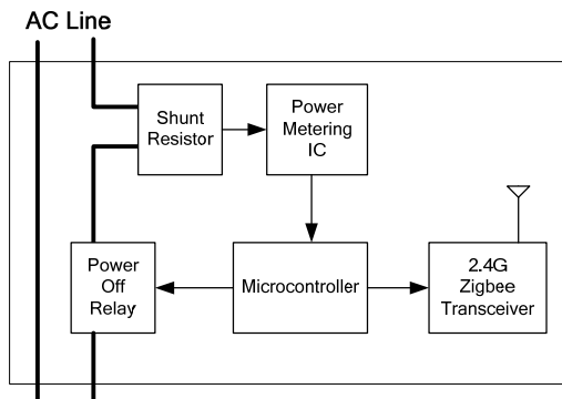
Fig. 2 Functional block diagram of ESD
