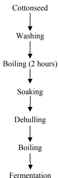
Fig. 2 Process Flow Chart for Cottonseed Fermentation
