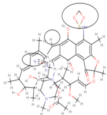
Fig. 7 (analog 57) N is replaced by CH_3 , carbonyl group( c=o ) by C\equiv N-CN and -OH by NHSO_2CH_2
