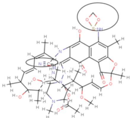
Fig. 6 (analog 8) -OH group is replaced by NHSO_2CH_2 & C=O by C\equiv N-CN
