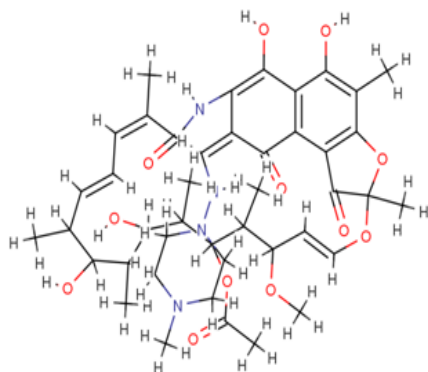
Fig. 4 RIFAMPICIN (CID:16043998) Molecular Formula: C_{43}H_{58}N_4O_{12} MW: 822.94022
