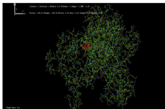
Fig. 12 Analog 35 docked with rpoB protein
