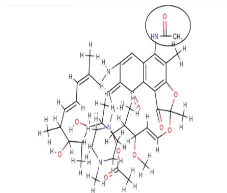
Fig. 5 (analog 1) -OH group is replaced by -NHCOCH_3 group
