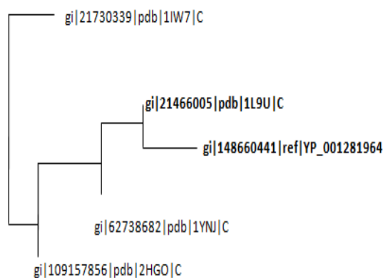
Fig. 1 Phenetic tree
