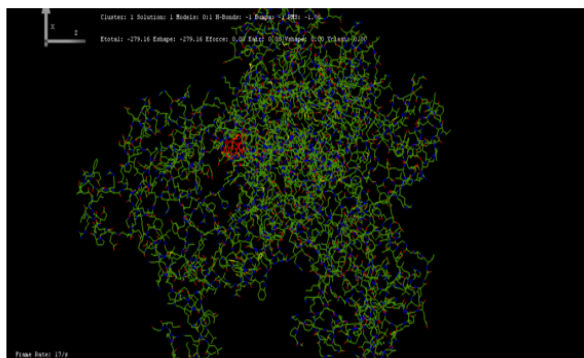
Fig. 9 Conventional Rifampicin (CID_16043998) docked with rpoB protein
