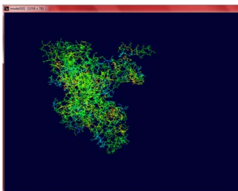
Fig. 2 rpoB viewed in SPDBV
