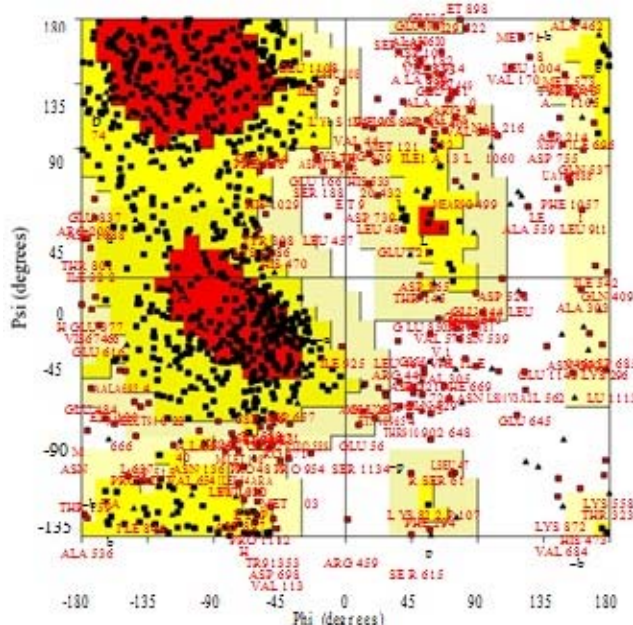
Fig. 3 Interactive Ramachandran Plot
